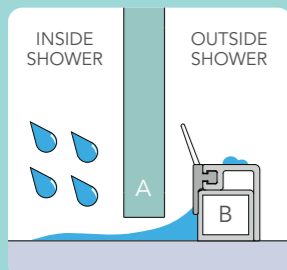
A - Sliding Door Glass B - Minimal Barrier Bar 1 - Threshold Seal
